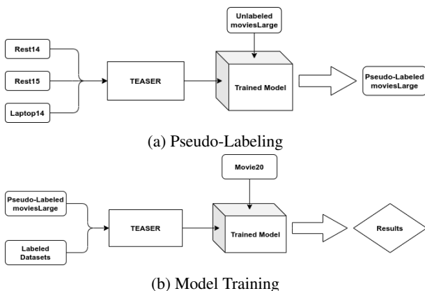
Figure 1: Semi-Supervised Learning: Model illustration
