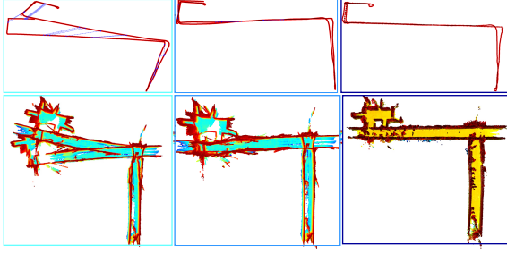
Figure 5: Rows represents pose graph and registered map. The first column corresponds to RTABMAP trajectory with robot revisiting the location from opposite view-points, blue dashed line represents early loop closures on pose graph, second and third column corresponds to optimized map based on VPR constraints and ground truth map respectively
