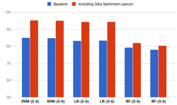
Figure 2: Accuracy improvements using Odia Sentiment Lexicon with Character-Level Features for Binary Classification
