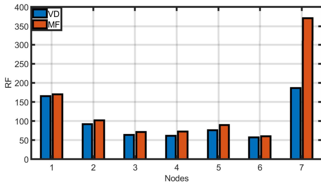
Fig. 4. PM10 sensing RF comparison for 7 Nodes for MAE=0.75
