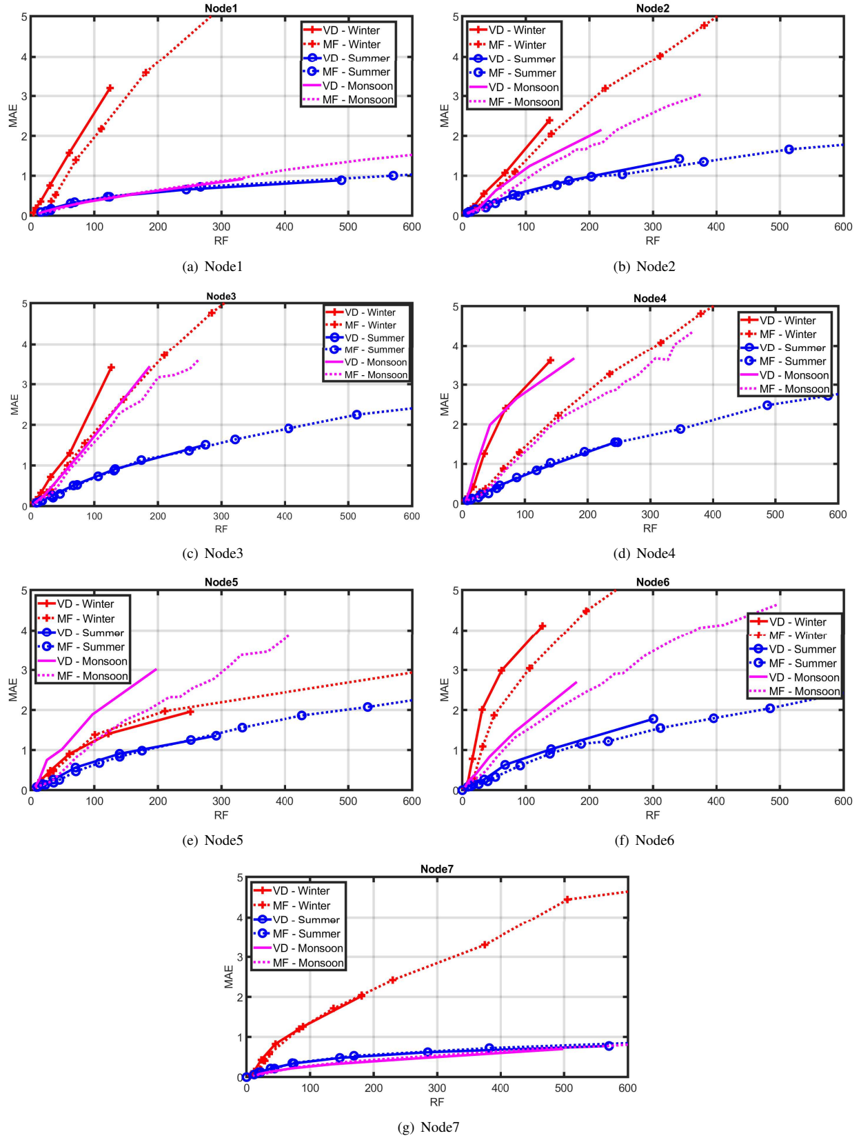
Fig. 2. RF v/s MAE - PM10 for seven Nodes
