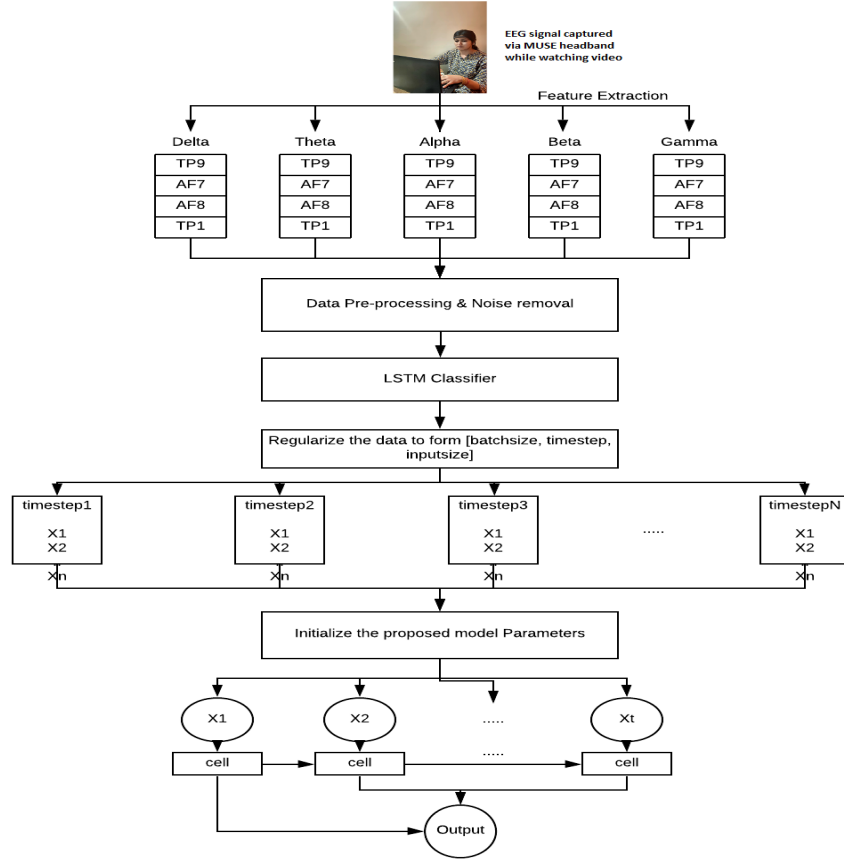
Figure 3: Proposed model for stress classification using EEG signals.
