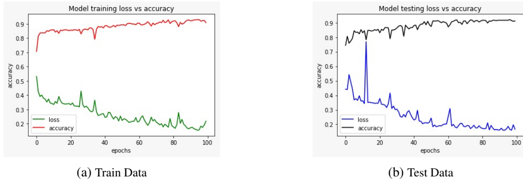
Figure 4: Model loss and accuracy with LSTM 2 architecture using 10-fold cross validation
