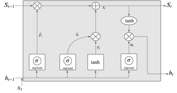
Figure 1: The basic architecture of an LSTM cell containing a forget gate, an input gate and an output gate.
