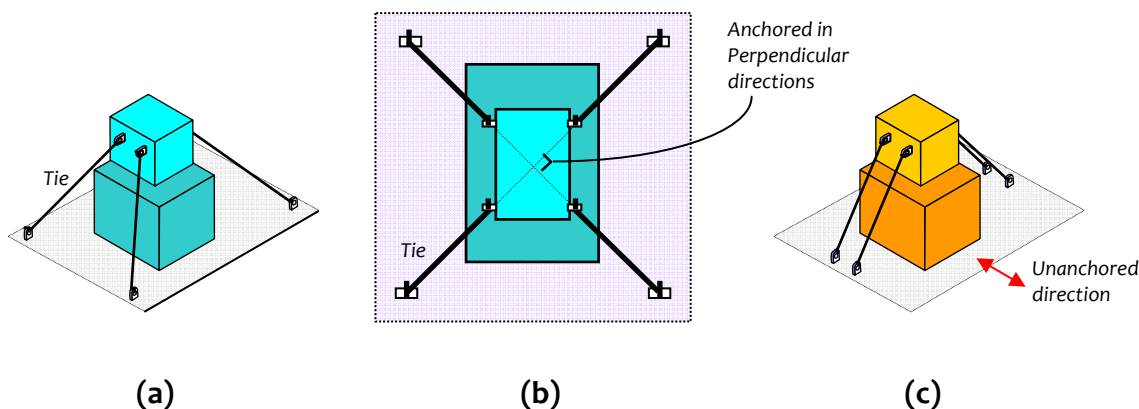
Figure 4.8: Direction of Tying NSEs: (a), (b) In any two perpendicular plan directions, NSEs must be tied; this will ensure that the object does not swing unrestrained in any direction, and (c) Otherwise, the NSE remains unanchored along one direction
