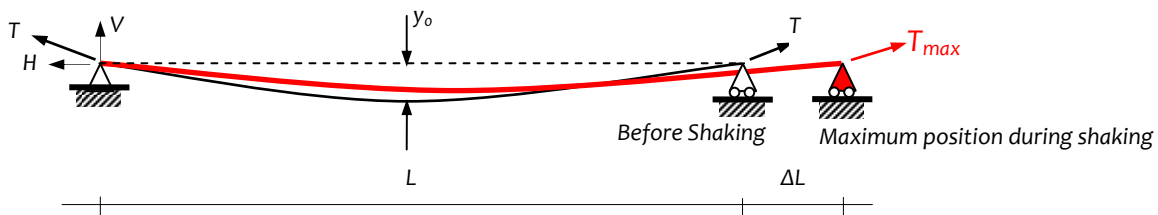
Figure B.11: Cable wire connected between building and pole: Tension, sag and extreme positions of cable before and during earthquake
