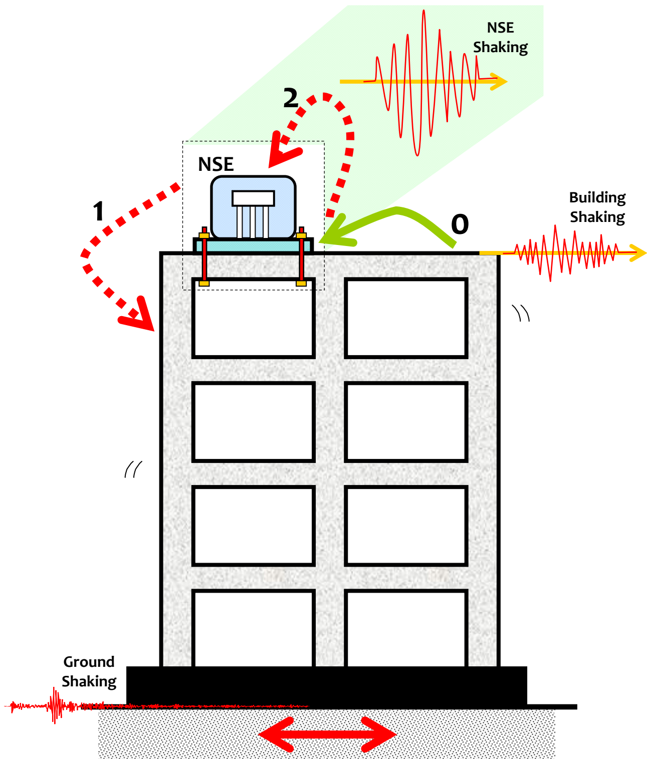
Figure 1.3: Various vibrations and interactions between SEs and NSE: There is no damage to NSE and feedback to building by the shaking of the NSE by the building
