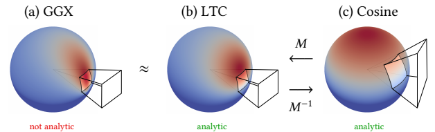
Figure 2: (a) A GGX lobe cannot be analytically integrated over the spherical domain covered by the area light. (b) An LTC represented by a matrix M provides a good approximation to the GGX lobe, and the integral equals (c) the analytic integral of a cosine lobe over the light transformed by M^{-1} .
