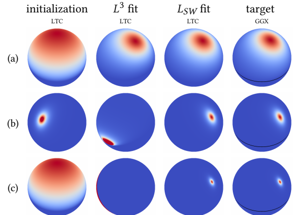
Figure 4: Fitting an LTC to a GGX lobe. We compare the L^3 fit of Heitz et al. to the L_{SW} fit we propose.
