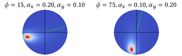
Figure 10: Roughness symmetries of the GGX BRDF. Permuting the x and y coordinates of the view vector and the roughnesses \alpha_x and \alpha_y produces the same permutation in the lobe's shape.
