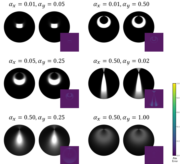
Figure 14: Rendered spheres with anisotropic materials and rectangular lights. We show the GGX reference (left), our LTC approximation (right), and the difference image. More results in our supplemental material.
