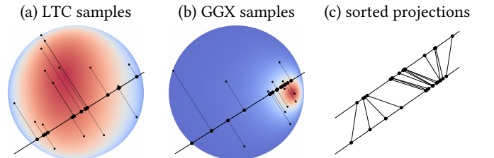
Figure 5: Illustration of Algorithm 3. We project random samples from the LTC (a) and the GGX lobe (b) onto a random direction and average the absolute differences between the sorted projections (c).
