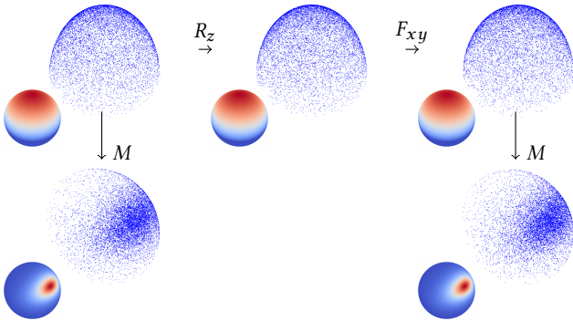
Figure 6: Non-uniqueness of LTCs. Cosine distributions remain unchanged under z -axis rotation R_z and xy flipping F_{xy} . Linearly transformed cosines inherit this invariance.
