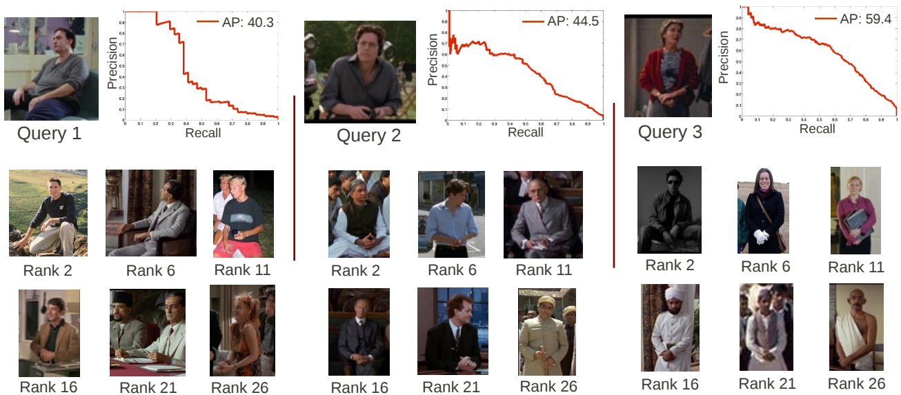
Fig. 8. Example retrievals: Top retrievals and AP curves for three queries are displayed. For the top retrievals every fifth sample from the top in retrieved list is displayed. The first mistake occurs at ranks 11, 4 and 33 respectively for the above queries.
