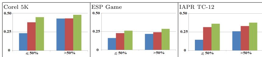
Fig. 2. Annotation performance in terms of mean recall (vertical axis) for the three datasets obtained using weighted KNN as in TagProp [3] (blue), using 2PKNN (red), and 2PKNN combined with metric learning (green). The labels are grouped based on their frequency in a dataset (horizontal axis). The first bin corresponds to the 50% least frequent labels and the second bin corresponds to the 50% most frequent labels.
