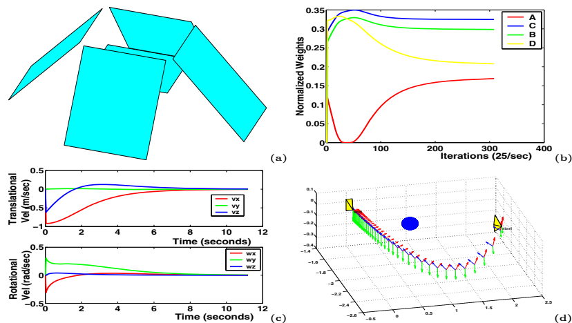
Fig. 4. (a) Non-Planar scene considered in the experiments. (b) Normalized weight values (c) Velocity Screw and (d) Camera Trajectory obtained for the scenario described in Fig. 3(a). Smooth convergence even in presence of degeneracies confirms the stable behavior of the proposed approach.
