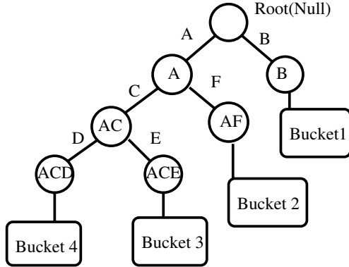
Figure 1. A Simple Bucket Trie
